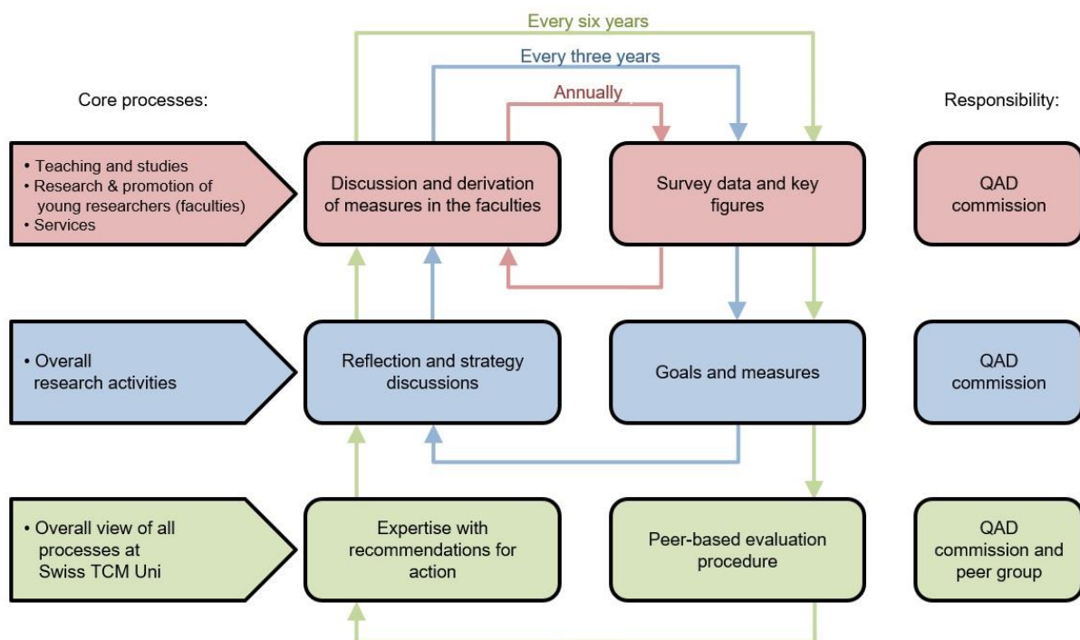
Figure 3: Evaluation cycles
